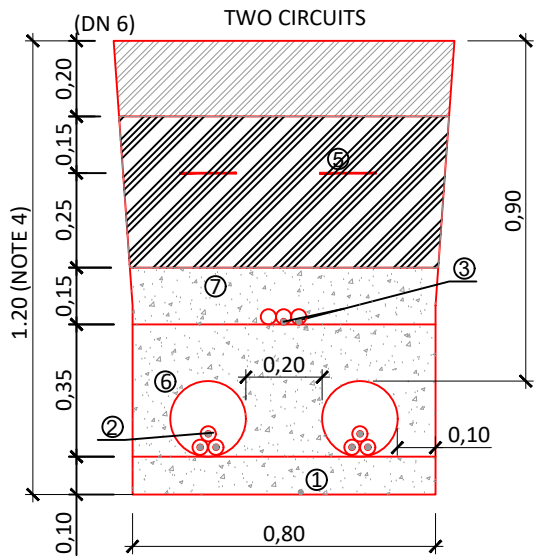
TRACK CROSSING TRENCH CROSS SECTION
