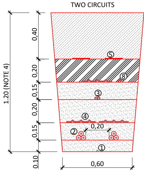
TRACK CROSSING TRENCH CROSS SECTION
